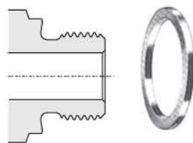
ISO Parallel with Metal Gasket Seal
